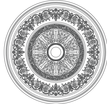
PLAS 826 CEILING ROSETTE 42-3/8" DIAMETER x 3-1/4" DEPTH 4-1/8" DIAMETER AT CENTER HOLE 3-1/4" DEPTH AT CENTER 6-1/4" DIAMETER FLAT AREA AT CENTER 60 LBS TOTAL WEIGHT (NOTE: ROSETTE IMAGE BELOW REDUCED)
